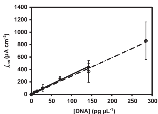
Fig. 5. Variation of the analytical signal with the concentration of DNA (●) from synthetic target (72 nt) and (○) from PCR amplicons (92 bp) using 3D-GNEE.
