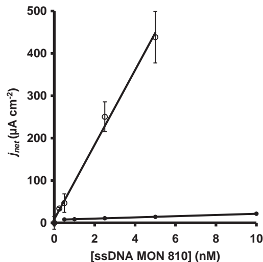
Fig. 4. Variation of the current density with the concentration of synthetic target (72 nt) using SPGE (●) and 3D-GNEE (○) under the optimized conditions up to 10 nM (SPGE) and 5 nM (3D-GNEE).
