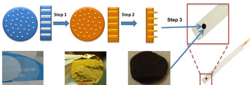
Fig. 1. Schematic representation of the fabrication of 3D-GNEE on polycarbonate membranes.
