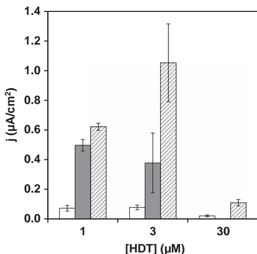
Fig. 3. Variation of the analytical signal expressed as density currents with the composition of the ternary monolayer obtained using 0.5 μM of CP and varying concentrations of HDT overnight. The concentration of MCH was fixed at 1 mM. White bars: blank experiment (no target). Gray bars: 5 nM of synthetic target (72 nt). Striped bars: 50 nM of synthetic target (72-nt). Other conditions as indicated in experimental section.
